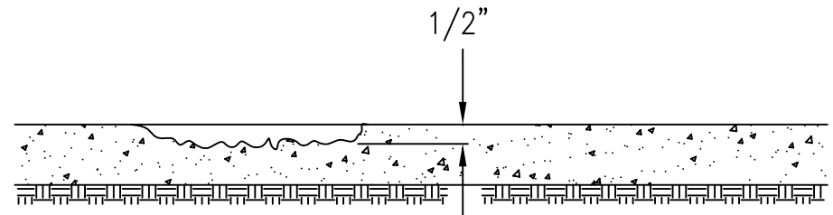
SPALLING OF SURFACE
