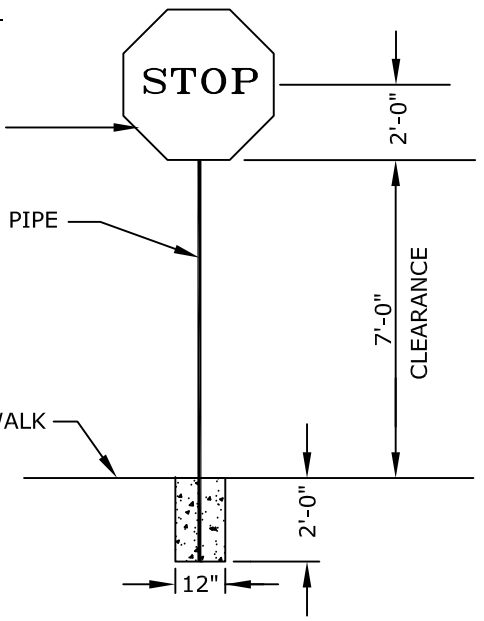
TYPICAL INSTALLATION
