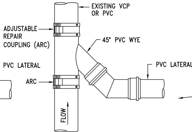
NEW WYE CONNECTION TO EXISTING VCP OR PVC SEWER
