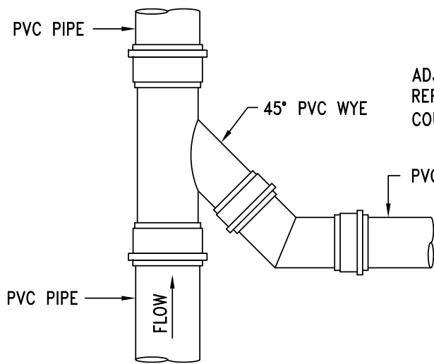
NEW WYE AND LATERAL NOT TO SCALE
